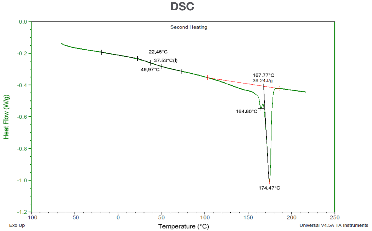
Figure 1. 2nd heating scan DSC data for the Nylon 12CF Flat (XY) sample.
